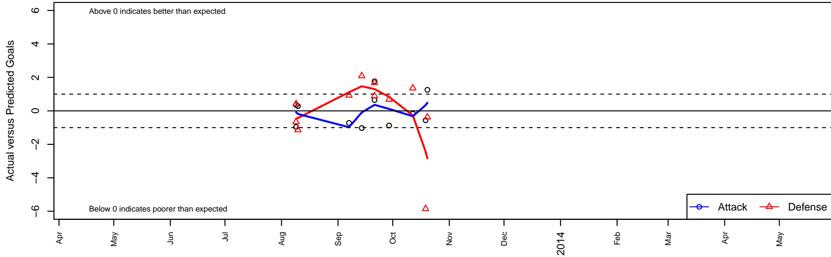
Central Cal SA White B02 Dots are actual minus expected GF (blue circles) and GA (red triangles). Blue line is smoothed change in attack strength. Red is smoothed change in defense strength.
